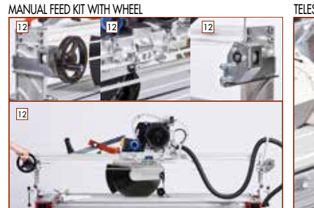
MANUAL FEED KIT WITH WHEEL
