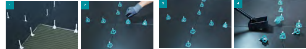
1 Place the level base under the tiles 10 cm from either end
