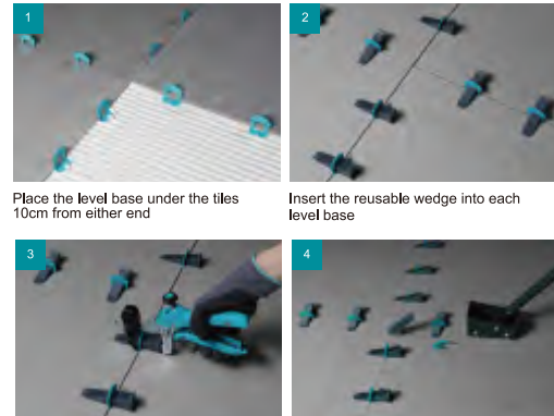
3 Use the plier to tighten to the required level
